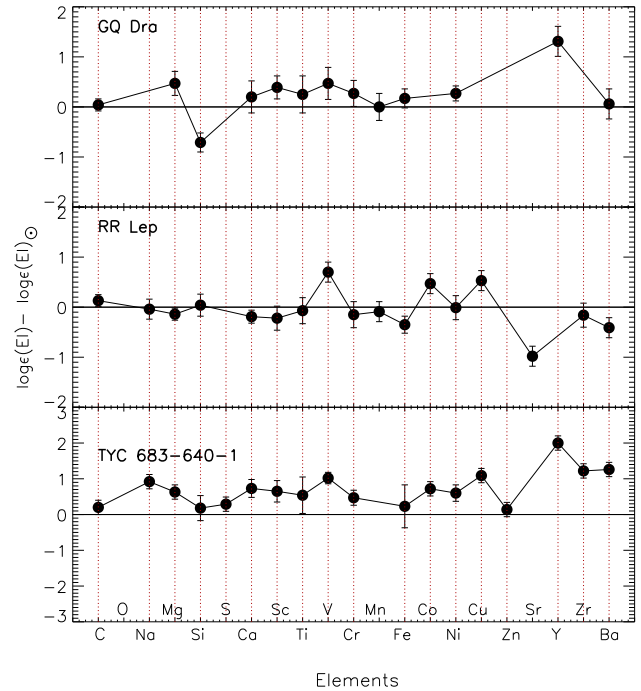
Figure 3. Chemical abundance distributions of the primary components of GQ Dra, RR Lep, and TYC 683-640-1 relative to solar chemical abundances (Asplund et al. 2009).
